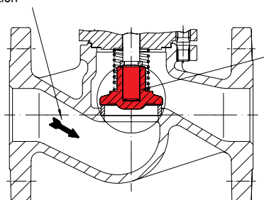
Hole and stem with a precise tolerance
