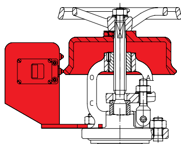
Limit switch
