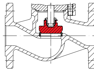
Plug with marginal seat
